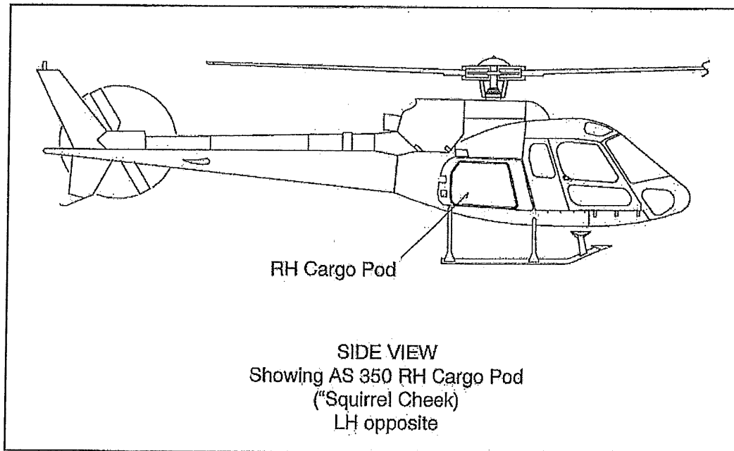
Figure 1 General Layout
