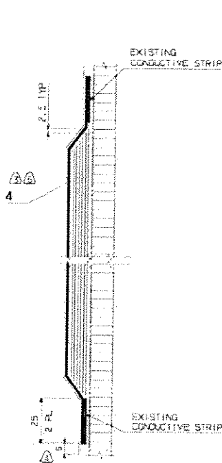
SECTION B-B
