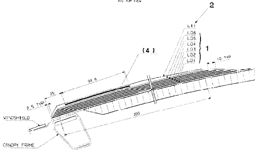
SECTION A-A LAY-UP SCHEME
