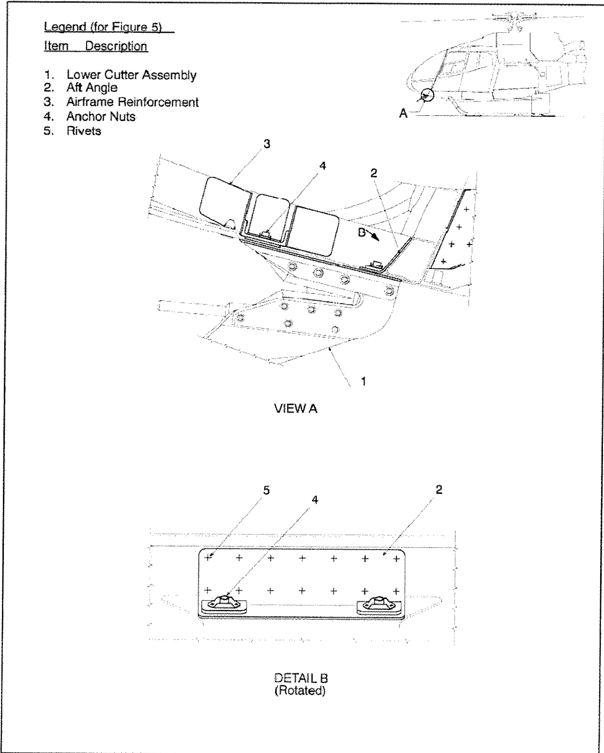
Figure 5 Lower Cutter Details
