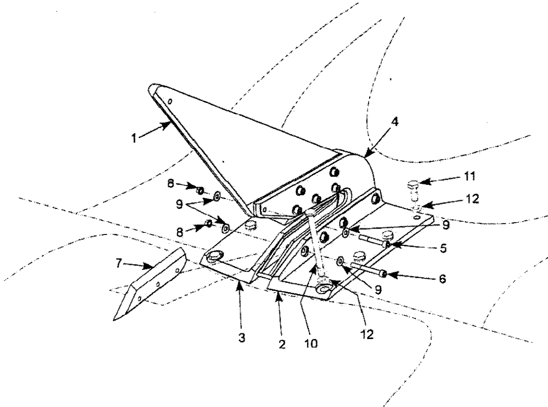
Figure 3-1 Upper Cutter Breakdown
