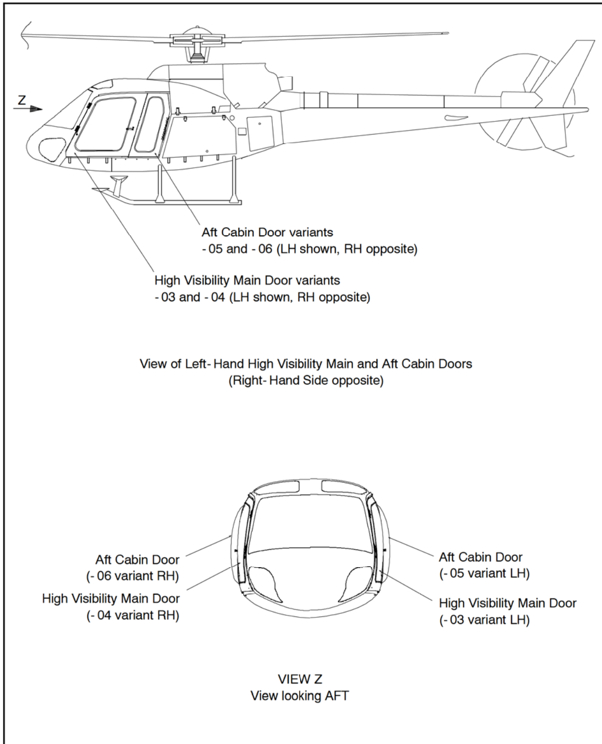
Figure 1 General Layout
