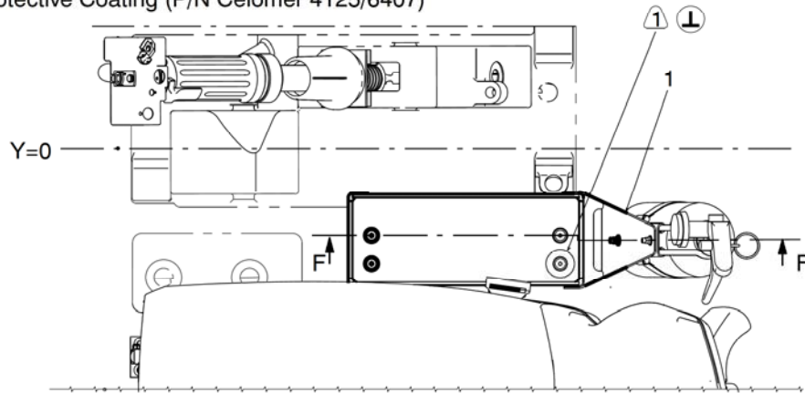
VIEW XX
