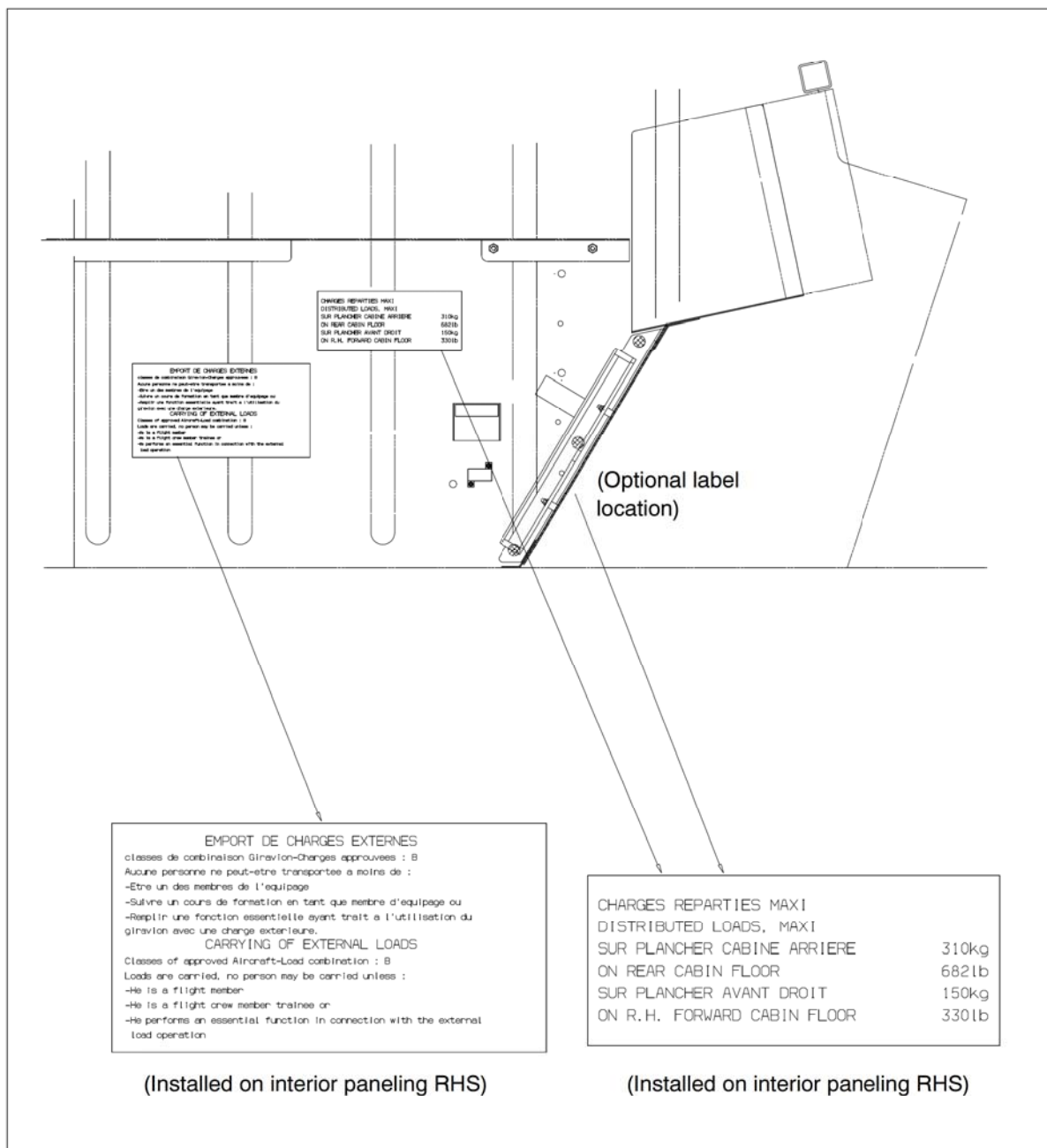
Figure 45 Identification label location in nosebay
