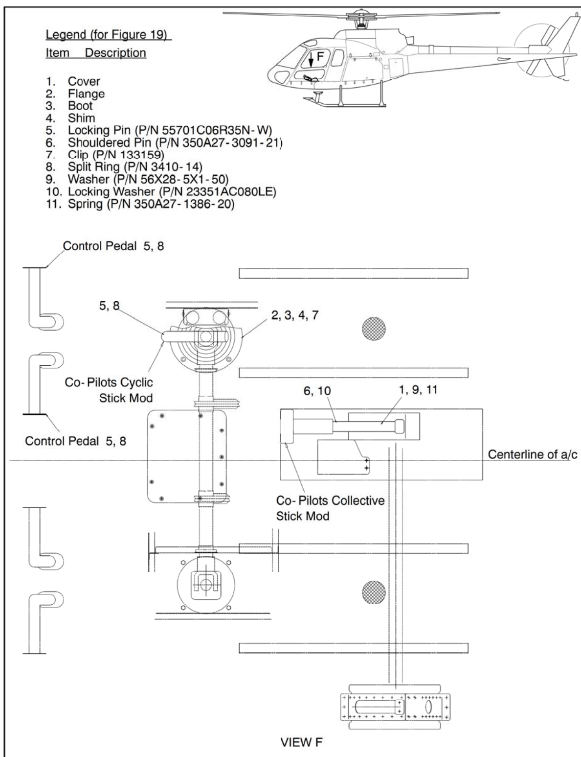
Figure 19 Dual Controls PRE & POST MOD AMS 07-3274
