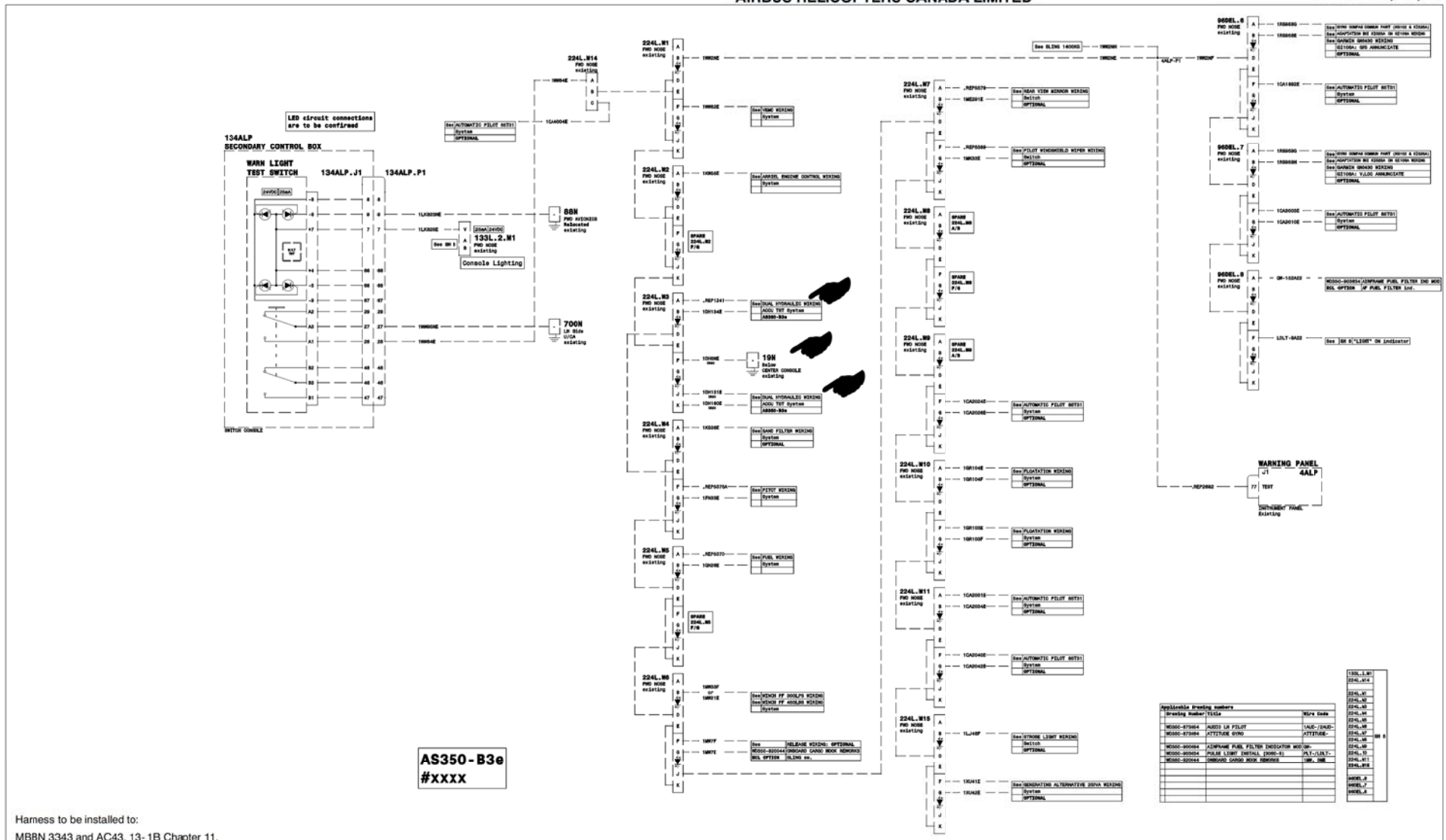
Figure 43 Instrument Lighting MOD, POST MOD AMS 07-4280, Page 5 of 8, Rev. B, Wiring Installation
