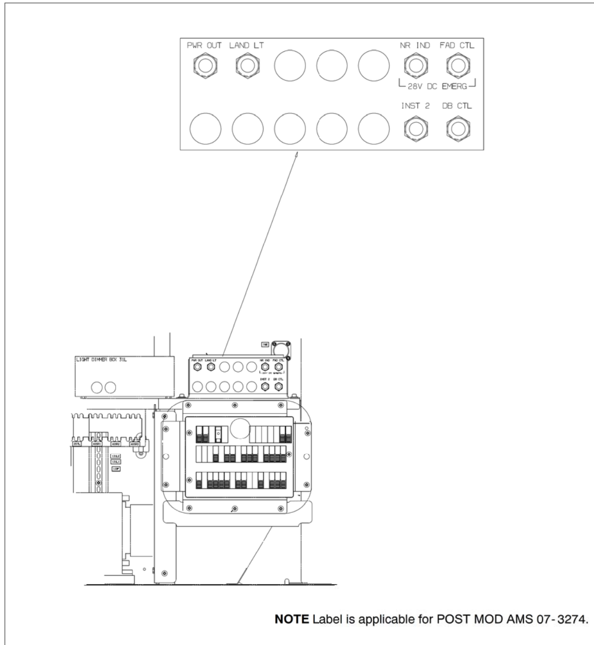
Figure 46 Identification label location in nosebay (AS 350 BA & B2)
