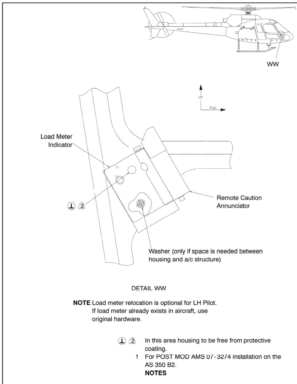
Figure 27 Load Meter Relocation and Remote Caution Annunciator System (AS 350 B2 & B3)
