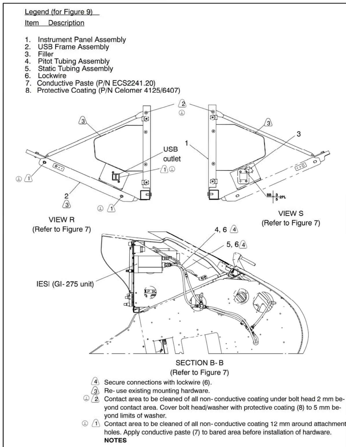
Figure 9 Instrument Panel MOD, POST MOD AMS 07-20112 (AS 350 B3) details
