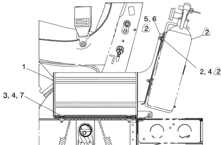
SECTION F-F
