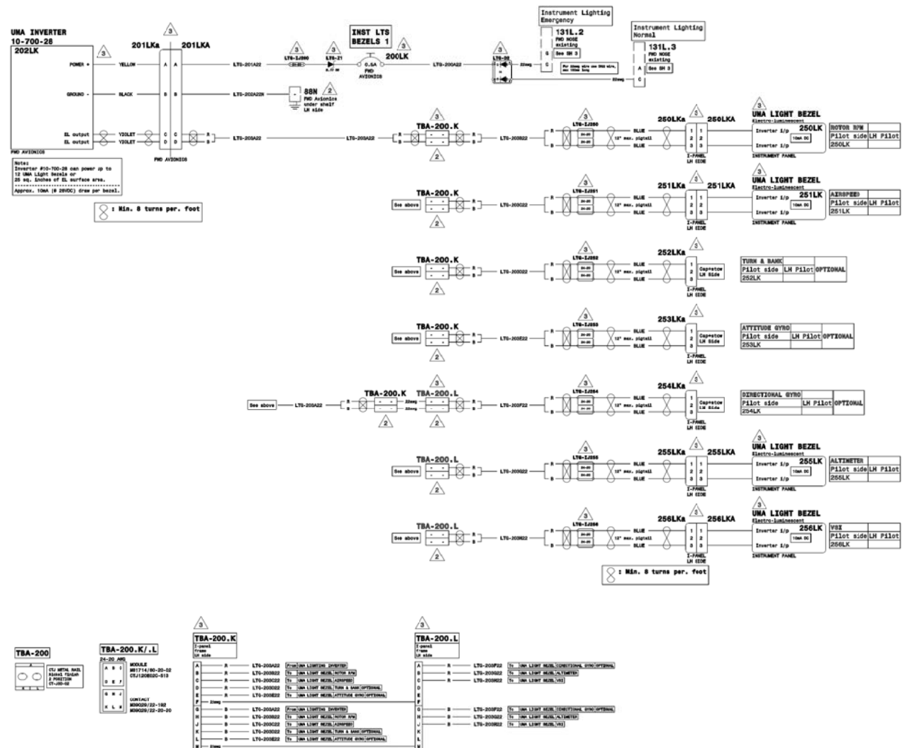
Figure 39 Instrument: Lighting MOD, POST MCD AMS 07-4280, Page 7 of 8, Rev. A, Wiring Diagram
