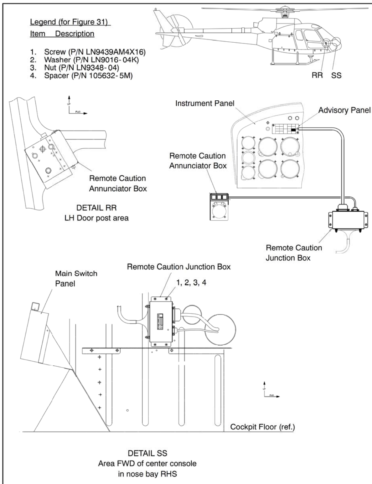
Figure 31 Remote Caution Annunciator System (AS 350 BA, B2 & B3)
