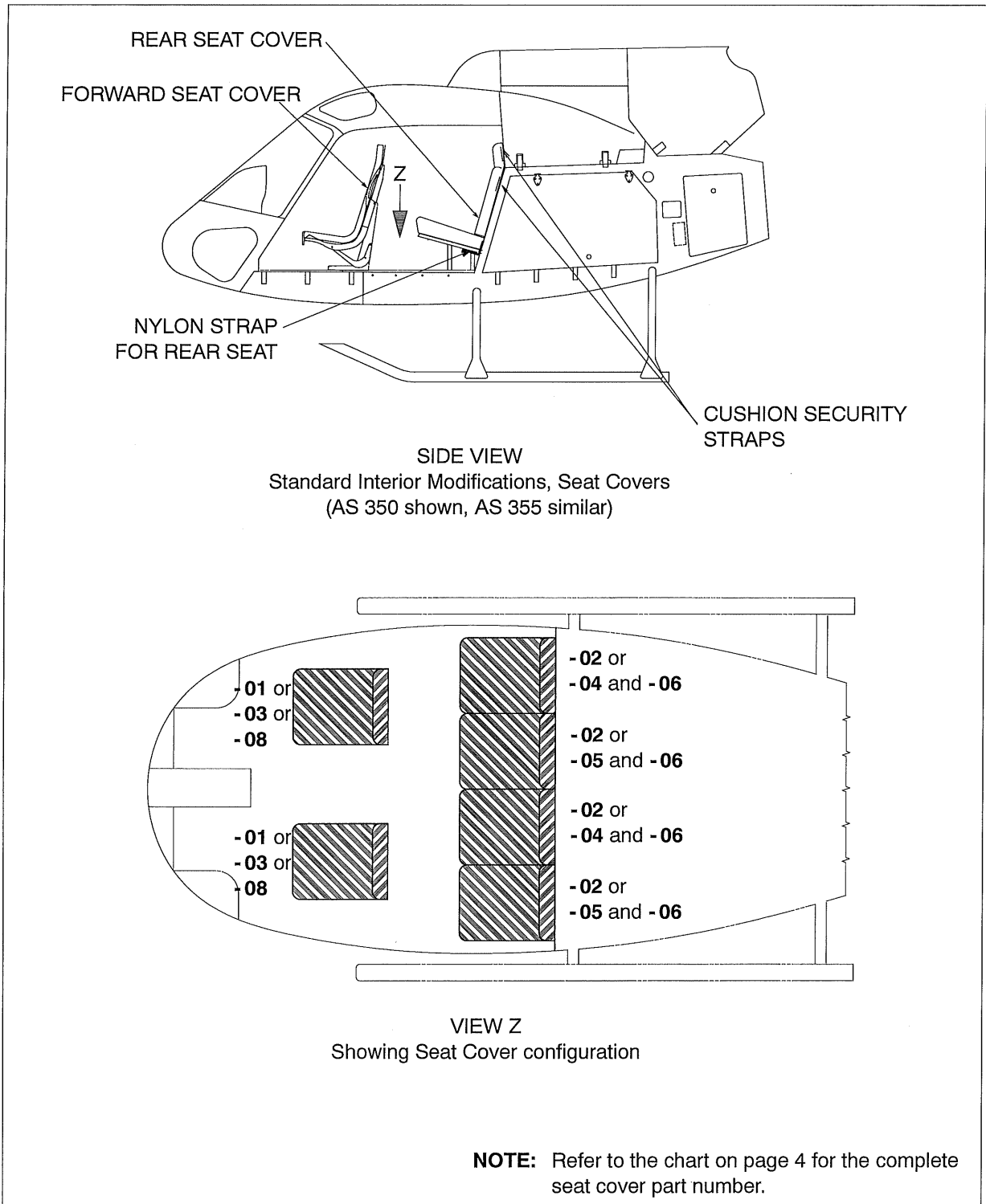
Figure 1 General Layout
