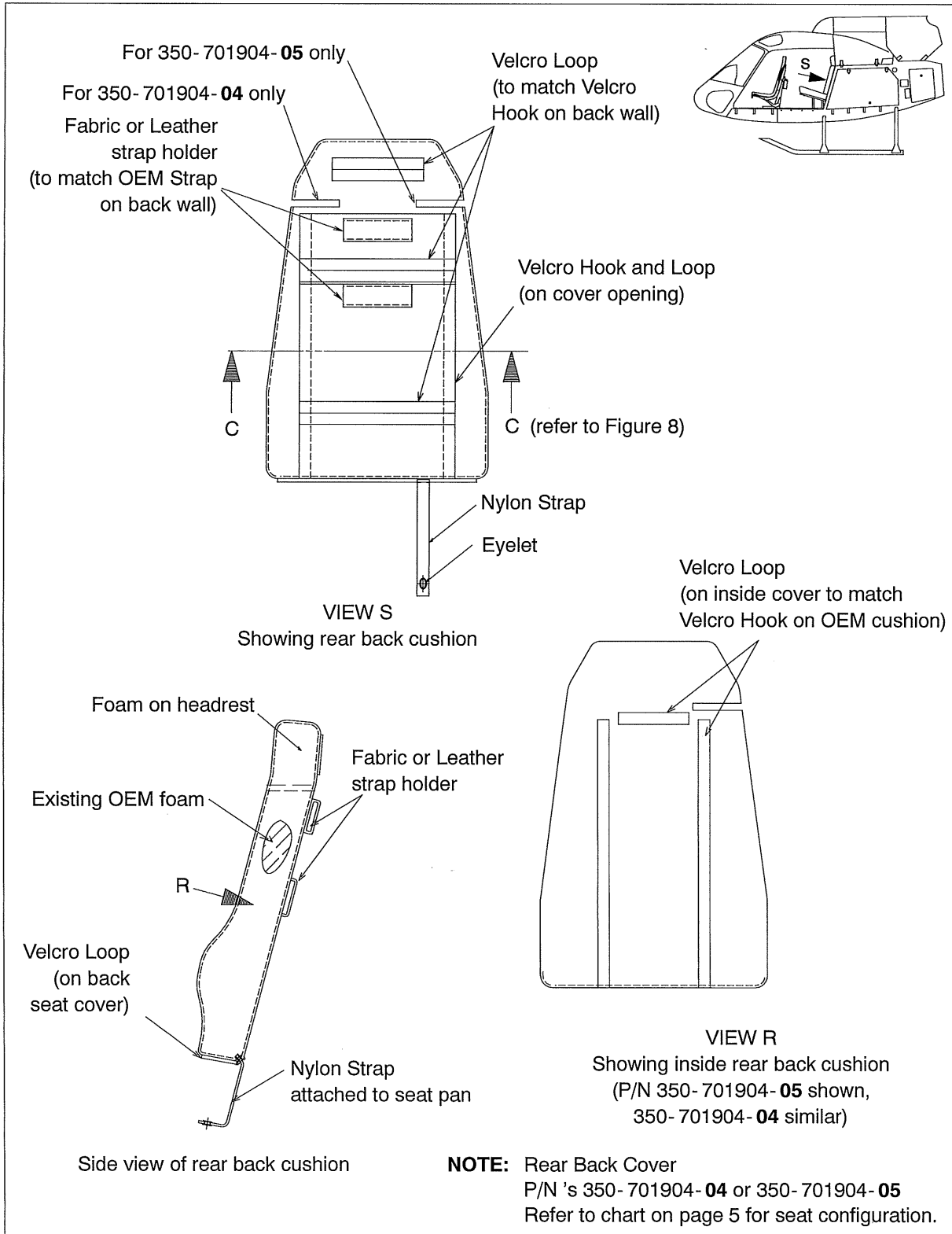
Figure 6 Rear Seat Cover Details for 350-701904-04 & -05
