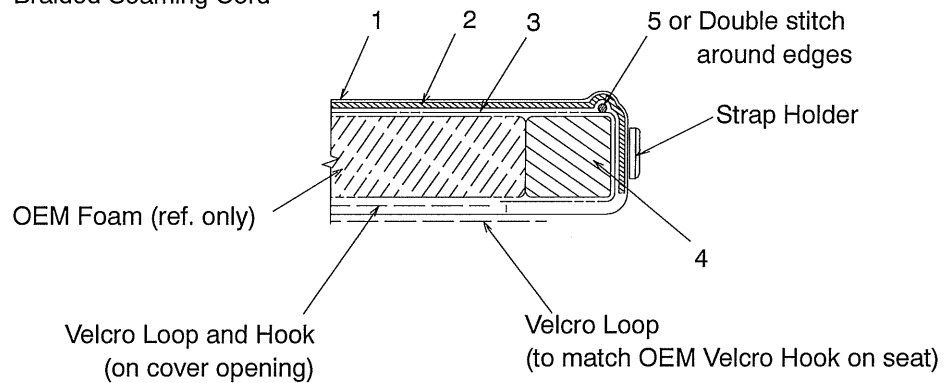
DETAIL T For rear bottom cushion
