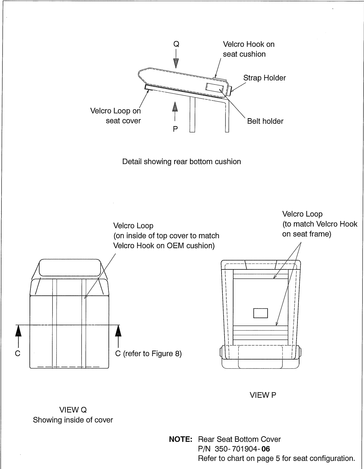
Figure 7 Rear Seat Cover Details for 350-701904-06
