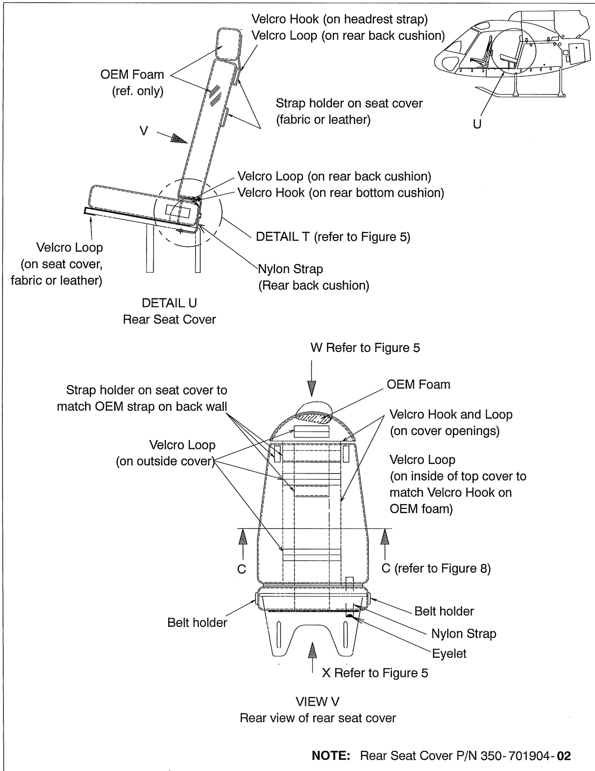
Figure 4 Rear Seat Cover Details for 350-701904-02
