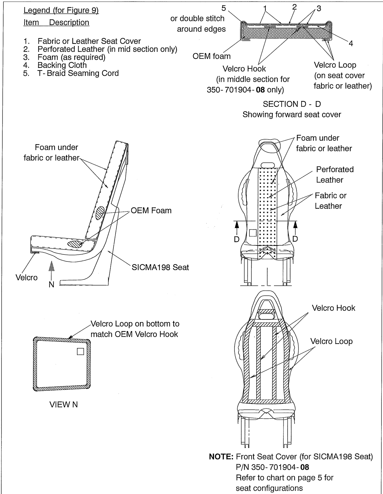
Figure 9 Forward Seat Cover Details for SICMA 198 Series Seat
