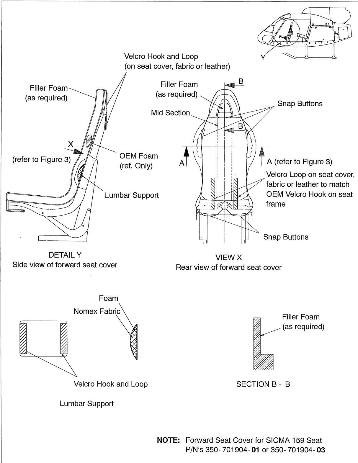
Figure 2 Forward Seat Cover Details for SICMA 159 Series Seat
