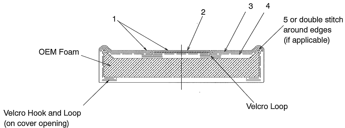
SECTION C- C Showing rear back and bottom seat cover
